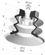
Sauggreifer 2.5 Falten Serie 96C Ø 30MM
