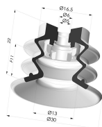
Bellows Suction Cup 2.5 folds Series 96C, Ø 30 mm
