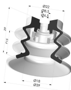
Bellows Suction Cup 2.5 folds Series 96C, Ø 40 mm
