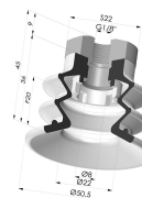
Bellows Suction Cup 2.5 folds Series 96C, Ø 50 mm
