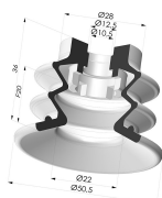
Bellows Suction Cup 2.5 folds Series 96C, Ø 50 mm
