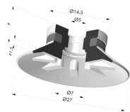
Flat Suction Cup Series 90, Ø 25 mm Product reference: 90 25-- A
