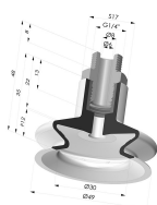
1.5 Bellows Suction Cup Series 8A Ø 49MM
