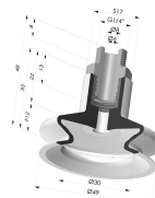
1.5 Bellows Suction Cup Series 8A Ø 49MM
