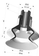
Bellows Suction Cup 1.5 folds Series 8A, Ø 44 mm
