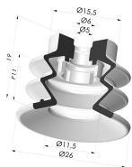
Bellows Suction Cup 2.5 folds Series 96C, Ø 25 mm
