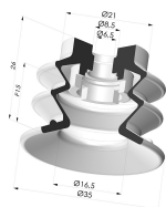
Bellows Suction Cup 2.5 folds Series 96C, Ø 35 mm
