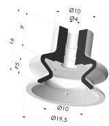
Bellows Suction Cup 1.5 folds Series 1, Ø 20 mm - With level on sealing lip
