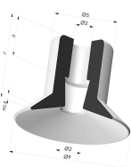
Flat Suction Cup Series 9, Ø 9 mm
