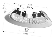
Flat Suction Cup Series 90, Ø 150 mm
