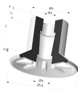
Flat Suction Cup Series 90, Ø 16.5 mm
