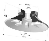
Flat Suction Cup Series 90, Ø 30 mm Product reference: 90 30-- A
