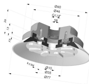
Flat Suction Cup Series 90, Ø 75 mm
