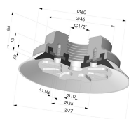
Flat Suction Cup Series 90, Ø 75 mm
