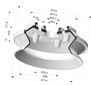
Bellows Suction Cup 1.5 folds Series 91, Ø 110 mm
