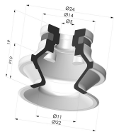
Bellows Suction Cup 1.5 folds Series 91, Ø 20 mm Product reference: 91 20-- A
