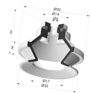
Bellows Suction Cup 1.5 folds Series 91, Ø 30 mm Product reference: 91 30-- A
