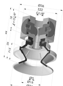
Bellows Suction Cup 1.5 folds Series 91, Ø 35 mm
