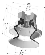
Bellows Suction Cup 1.5 folds Series 91, Ø 35 mm
