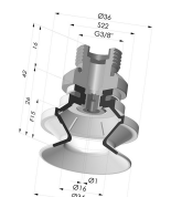
Bellows Suction Cup 1.5 folds Series 91, Ø 35 mm
