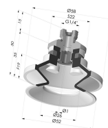
Bellows Suction Cup 1.5 folds Series 91, Ø 50 mm
