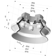
Bellows Suction Cup 1.5 folds Series 91, Ø 75 mm
