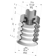
Bellows Suction Cup 4.5 folds Series 92, Ø 20 mm Product reference: 92 20-- 18
