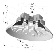
Flat Suction Cup Series 94, Ø 100 mm
