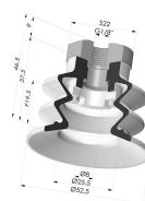
Bellows Suction Cup 2.5 folds Series 96, Ø 52 mm
