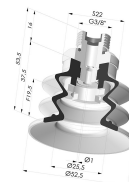
Bellows Suction Cup 2.5 folds Series 96, Ø 52 mm
