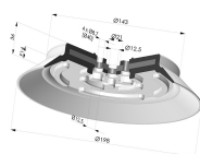
Flat suction cup series PFG, Ø 198 mm
