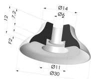
Flat suction cup series PFG, Ø 30 mm
