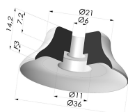
Flat suction cup series PFG, Ø 36 mm
