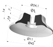
Flat suction cup series PFG, Ø 42 mm
