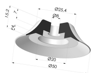
Flat suction cup series PFG, Ø 50 mm
