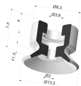
Flat suction cup series PFG Ø 10.5 mm
