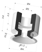
Flat suction cup series PFG, Ø 4 mm
