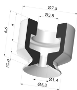
Flat suction cup series PFG Ø 5.3 mm
