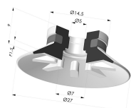
Flat Suction Cup Series 90, Ø 25 mm
