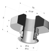
Separable Female Fitting 1/8G
