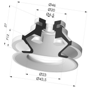
Bellows Suction Cup 1.5 folds Series 91, Ø 40 mm Product reference: 91 40-- A
