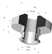
Separable Female Fitting 1/8G Product reference: 9G18-2
