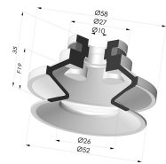
Bellows Suction Cup 1.5 folds Series 91, Ø 50 mm Product reference: 91 50-- A
