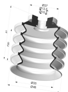
Bellows Suction Cup 4.5 folds Series 92, Ø 50 mm
