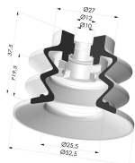
Bellows Suction Cup 2.5 folds Series 96, Ø 52 mm
