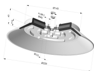
Flat suction cup series PFG, Ø 225 mm
